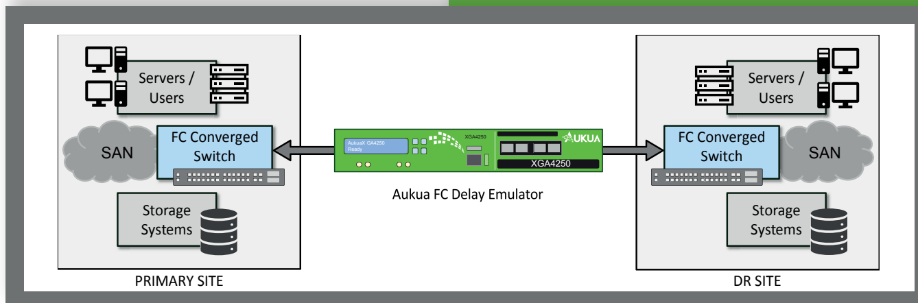
Figure 2: Fibre Channel distance emulation setup with the Aukua FC Delay Emulator
